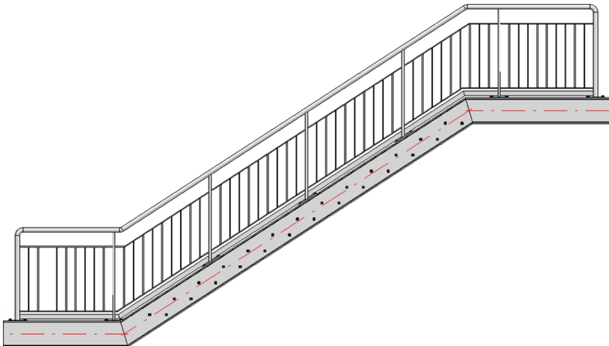
Example: Distribution of posts across complete walking distance (different at transitions)
