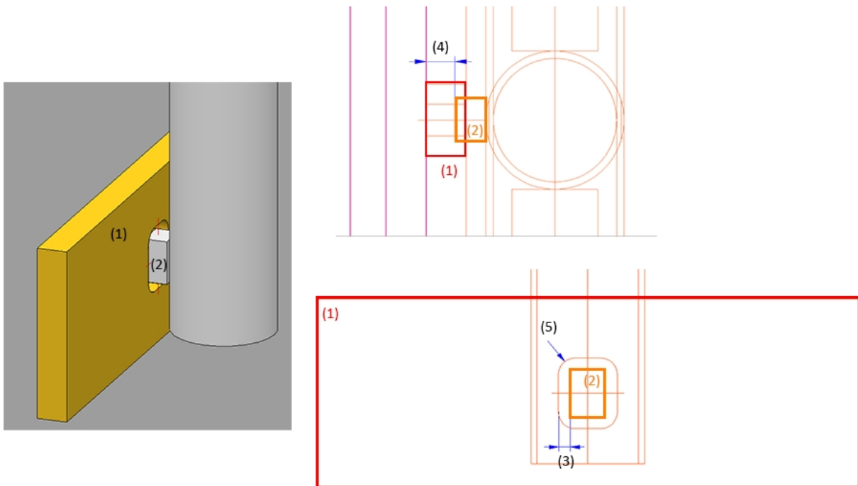
(1) Base plate, (2) Distance element, (3) Clearance, (4) Offset, (5) Corner radius
