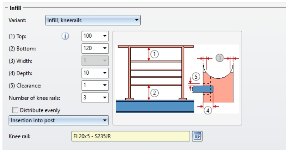
Value inputs for knee rails
