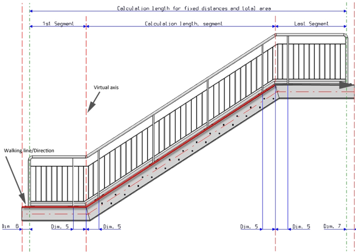
Example: Distribution of posts across complete walking distance (different at transitions)
